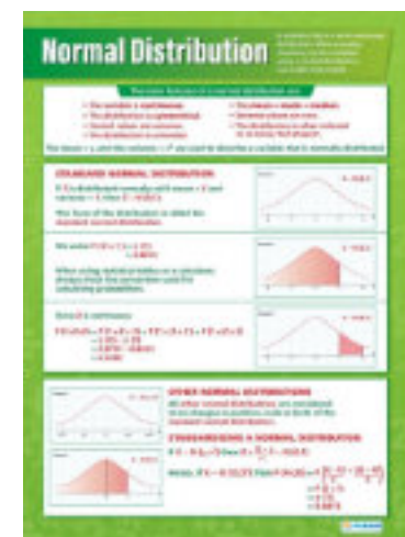
Normal Distribution
